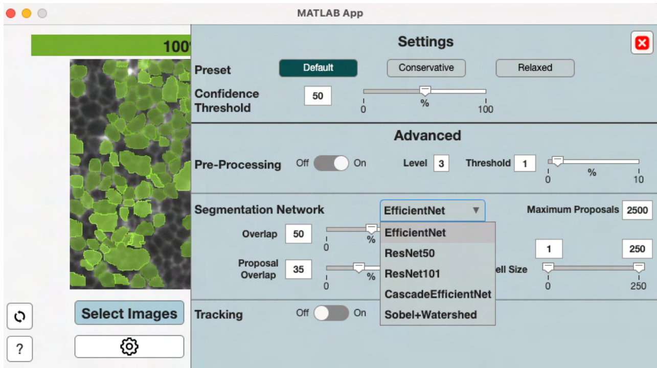
Figure 10. S+W algorithm added into the drop down menu among other Deep Learning algorithms.
