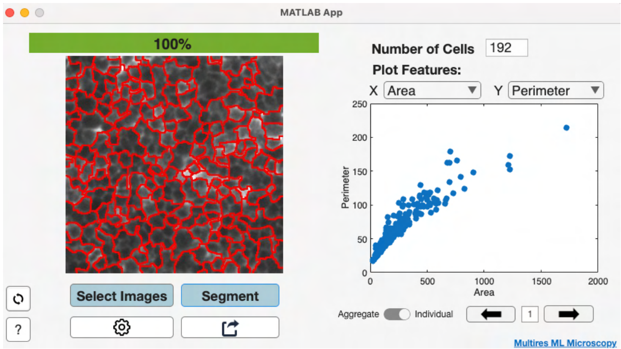
Figure 12. S+W segmentation completed in the GUI.
